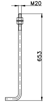
4 x M20 x 720 Anchor Bolts
