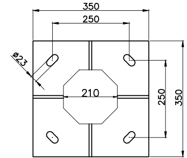
Base Plate # 14 mm x 350 x 350
